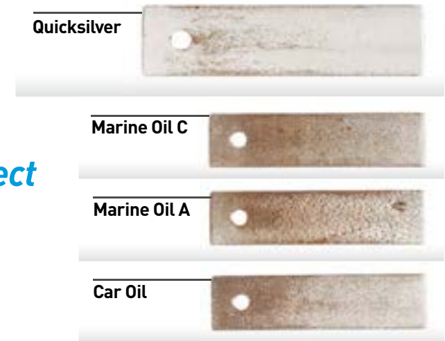
Saltwater / 100% Humidity NMMA FC-W Rust Test
