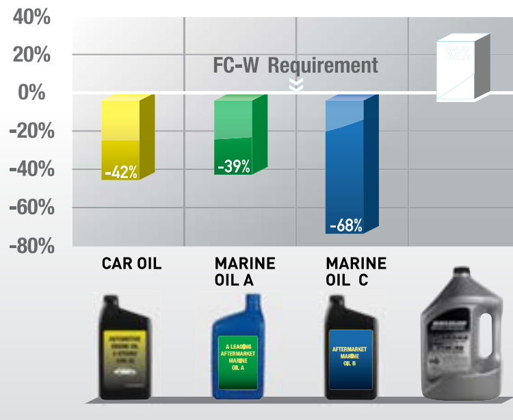
NMMA FC-W Rust Test
