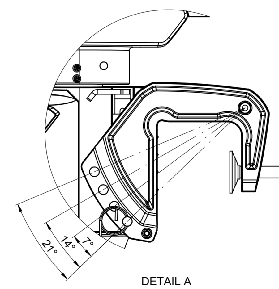
DETAIL A
