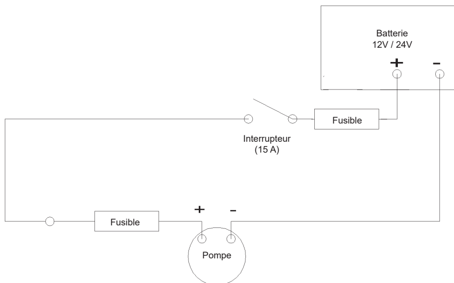
Fig. 5 Raccordements
