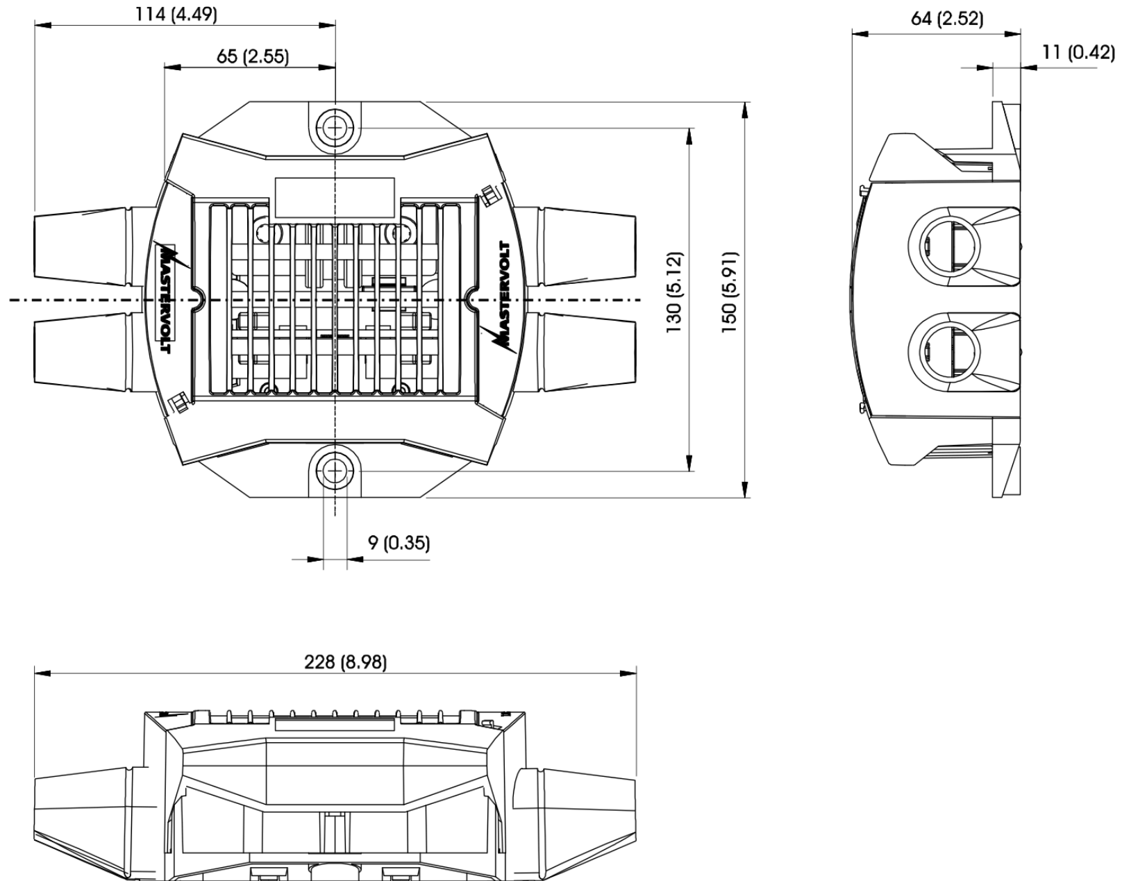
Figure 5: Dimensions MasterShunt 500 in mm [inches]
